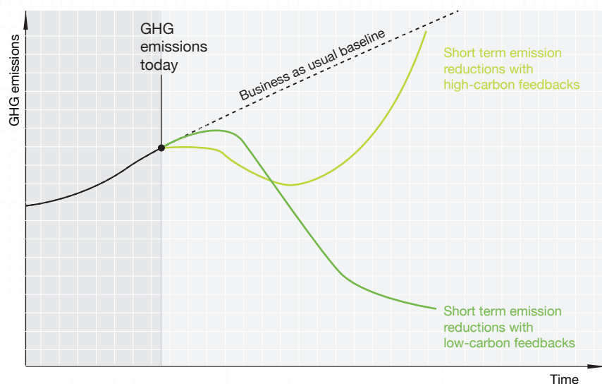
GHG emission pathways with Biotech
